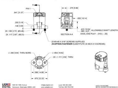
M3K Magnetic Kit Encoder (5-Option Bolt Circle)
