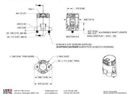
M3K Magnetic Kit Encoder (5-Option Bolt Circle)
