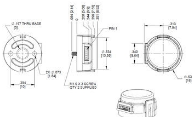
E16 Micro Optical Kit Encoder
