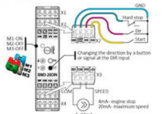
DC brush motor speed control using analog signal 4...20 mA. Connection diagram
