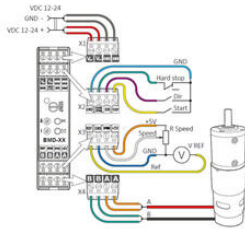
Connection of the DC brush motor speed controller BMD-501R
