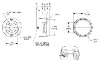
E16 Micro Optical Kit Encoder
