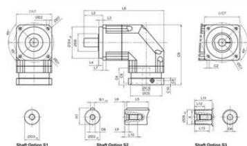
Dimensions (1-stage, Ratio i=3~20) / ABR Series
