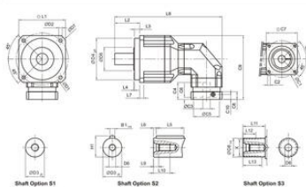
Dimensions (2-stage, Ratio i=15~200) / ABR Series
