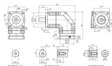
Dimensions (1-stage, Ratio i=3~20) / ABR Series
