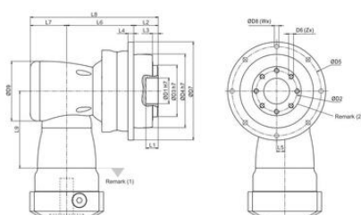
Dimension - MDK (2 Stage) Gearbox (Ratio i = 12 \sim 100 )
