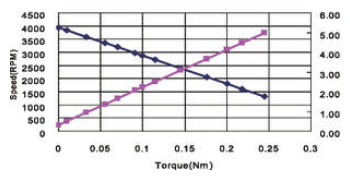
MB054TP100 CURVE
