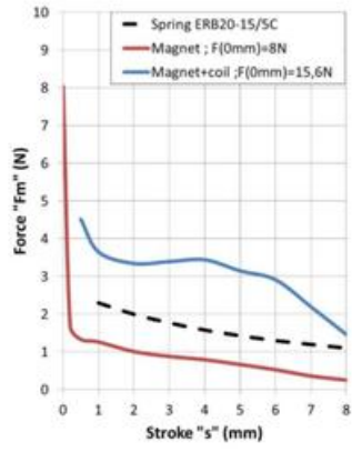
Force-stroke curve (F-S)
